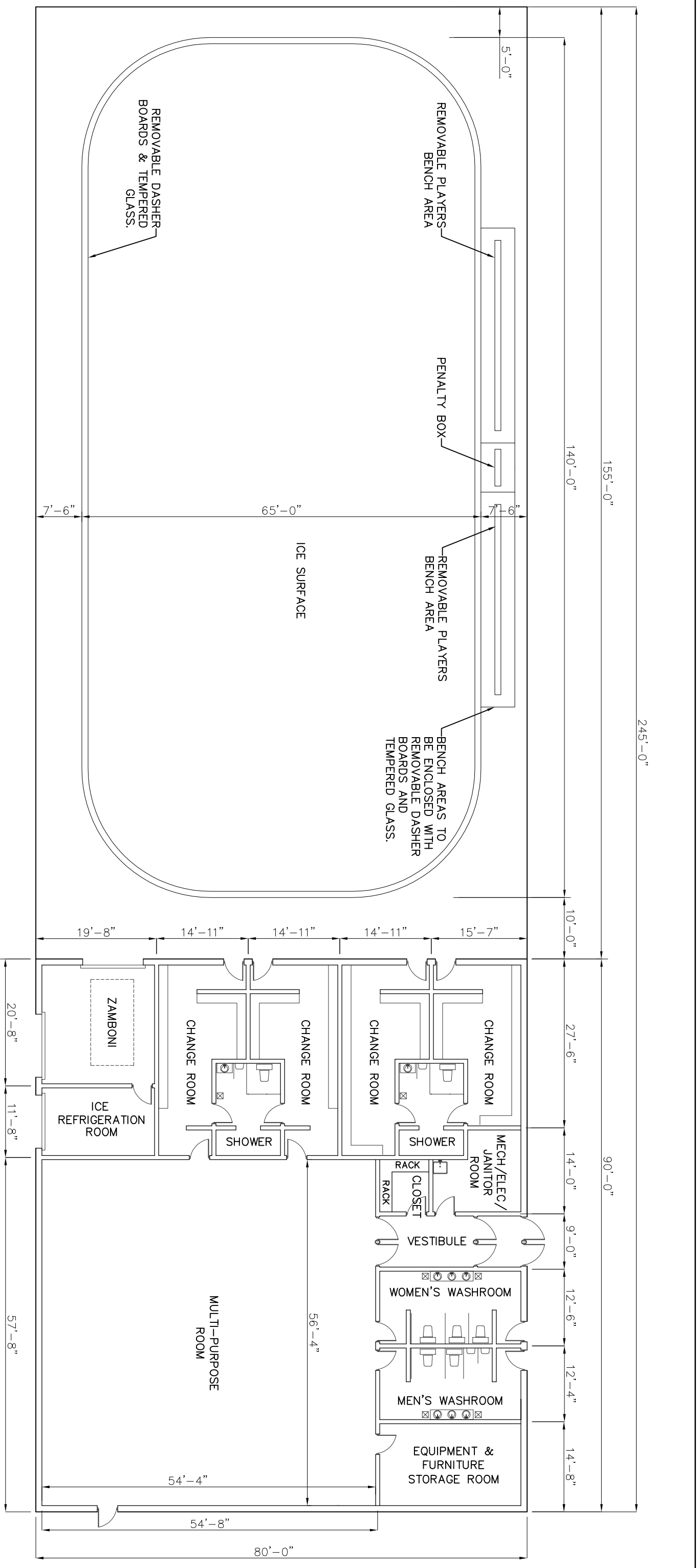
FLOOR PLAN SCALE: 1/16" = 1'-0"
